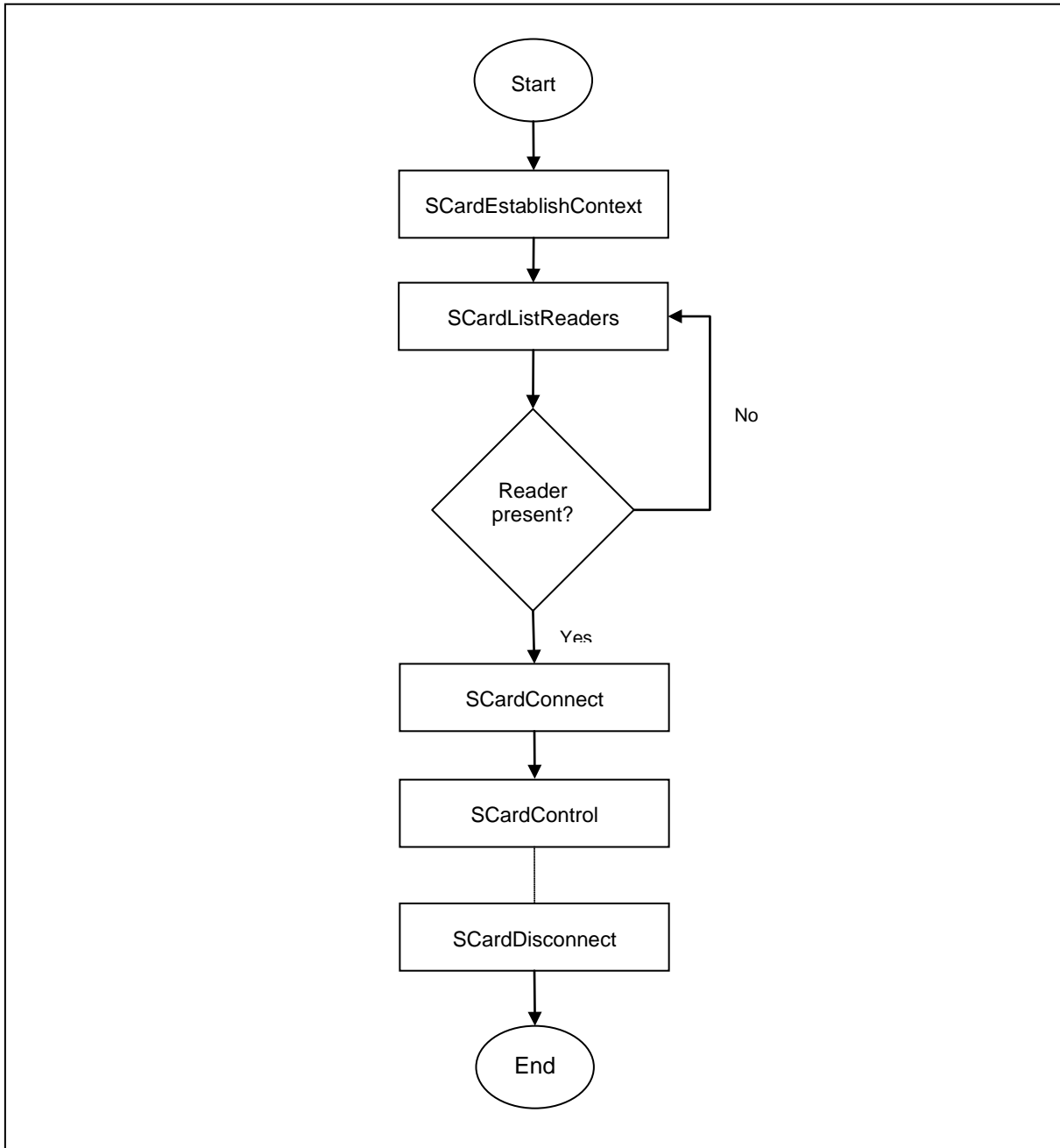
Figure 3: ACR1252U-A1 Escape Command Flow
