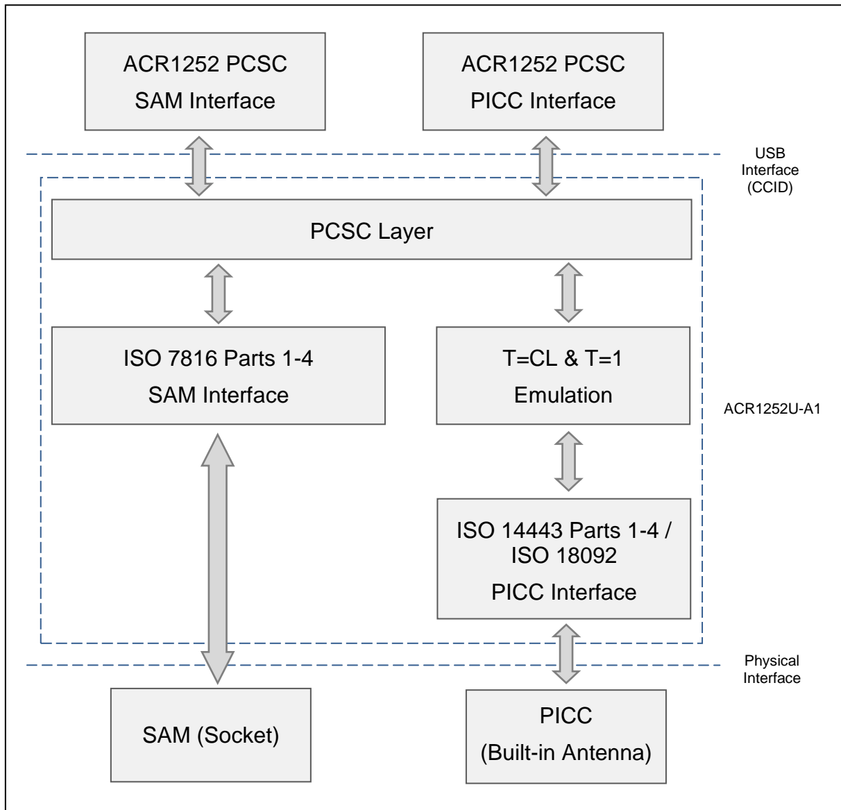
Figure 1: ACR1252U-A1 Architecture
