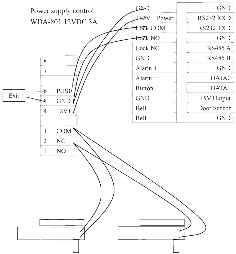
Figuration: F7/F708 to control the electrical locks
